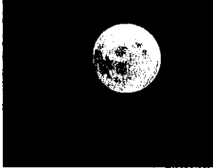
The Moon
